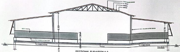
SECTIONAL ELEVATION A-A
